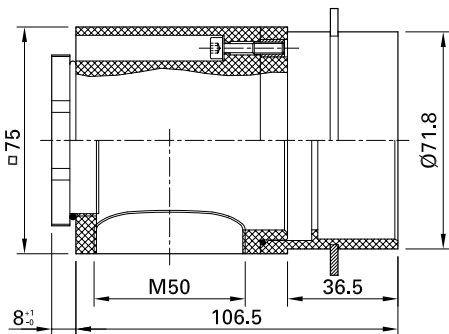
MGK4VB10-14+MGK4R-M50
