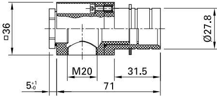
MGK1VB10-14+MGK1R-M20
