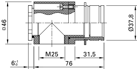
MGK2VB10-14+MGK2R-M25
