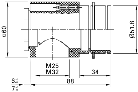
MGK3VB10-14+MGK3R-M...
