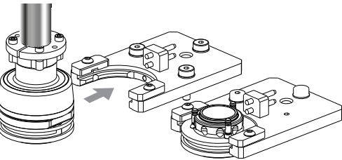
Automatic operation
